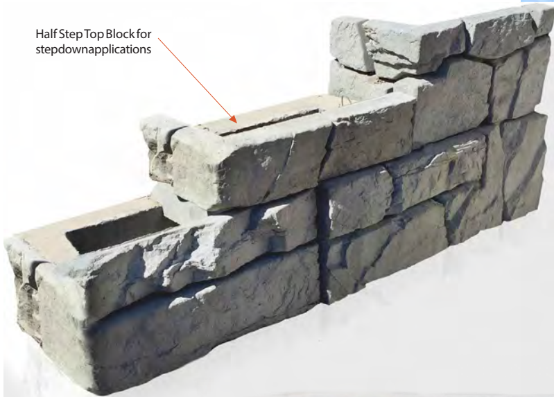
Double-Sided Verti-Block parapet wall with 6" Cap
